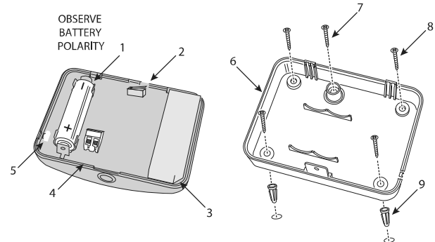
Figure 2 Wireless Indoor Repeater Component and Feature Locations
